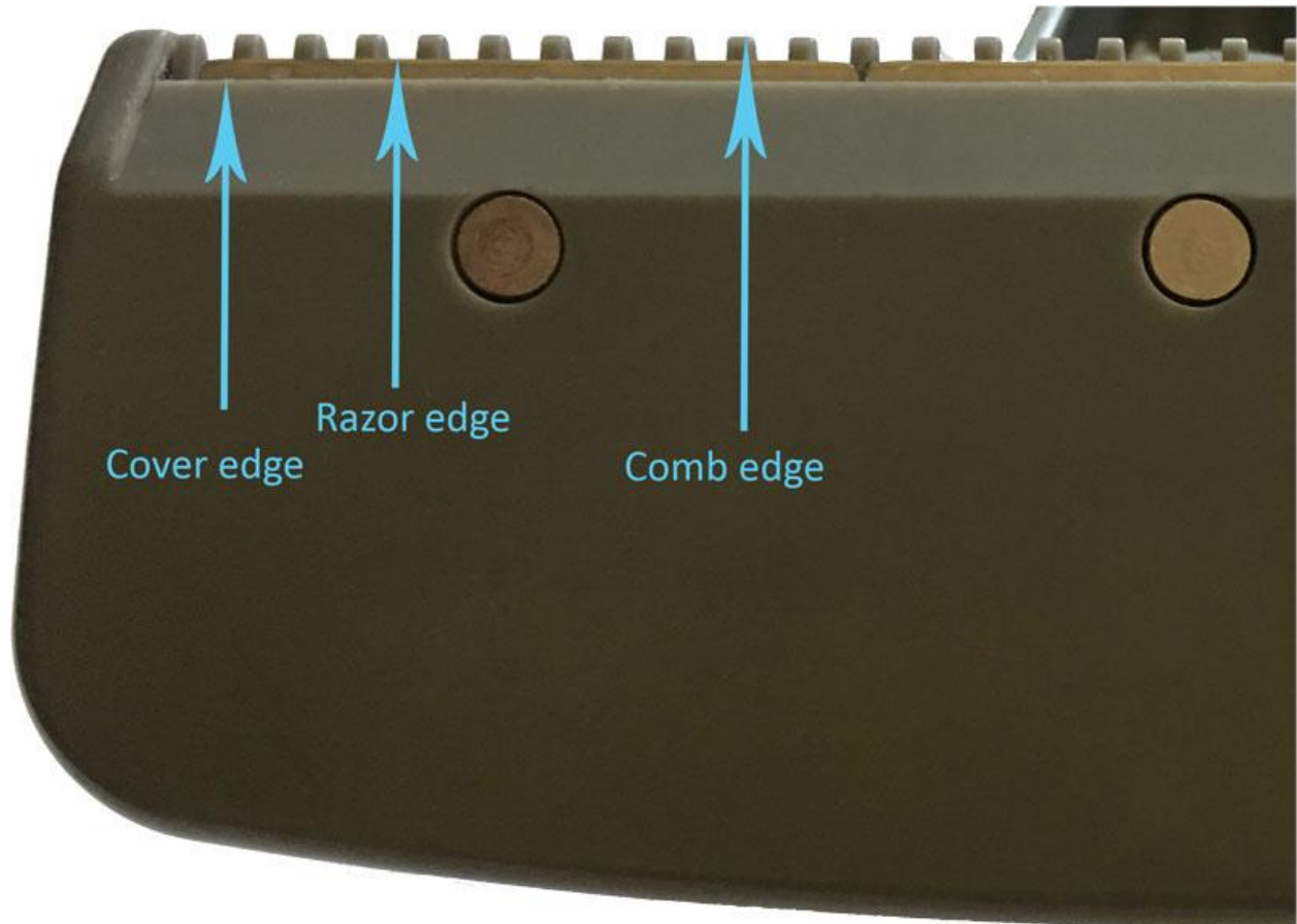
Figure 2. Razor edge is guarded between Comb edge and Cover edge.
